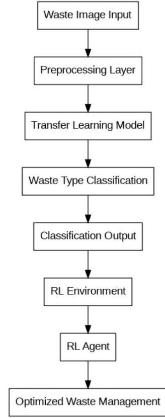
Fig. 4. System's Architecture for Waste classification and optimization
